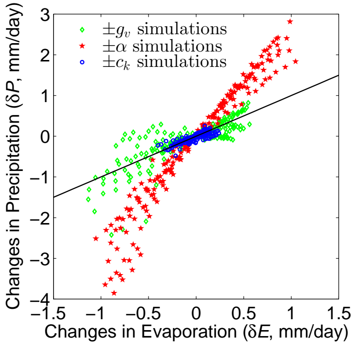
Figure 4-11: Scatter plot of changes in precipitation ( \delta P , mm/day) against changes in evaporation ( \delta E , mm/day), for RC model simulations with no cloud-radiation interactions or diurnal cycle. The black diagonal line indicates \delta P = \delta E , which is followed roughly for \pm g_v and \pm c_k simulations, but not \pm \alpha simulations, where precipitation changes much more rapidly than evaporation due to changes in overturning circulation strength.
