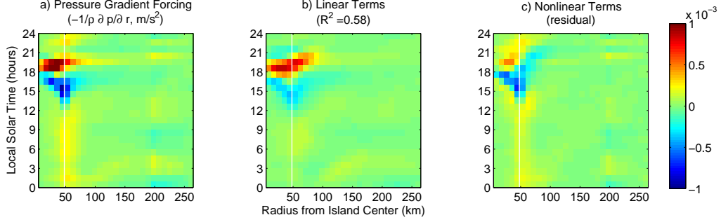
Figure 5-12: Radially and diurnally composited plot of the terms in the radial momentum budget for surface winds, in the reference-case island simulation (radius:left-to-right, local solar time: bottom-to-top). Subplots show a) Pressure gradient acceleration ( \text{m/s}^2 ), b) linear terms in surface wind radial momentum equation ( \partial u_r / \partial t + \alpha u_r ) and c) the inferred sum of nonlinear terms in the radial momentum equation; see Equation (5.3). The majority of the variance in the pressure gradient acceleration is explained by the sum of the linear terms.
