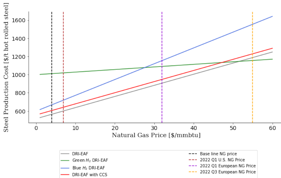
Figure 3-11: Steel production cost sensitivity to natural gas
