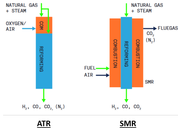
Figure 2-1: Simplified figures of the ATR and SMR processes. Figure from Sadler & Anderson (2018)
